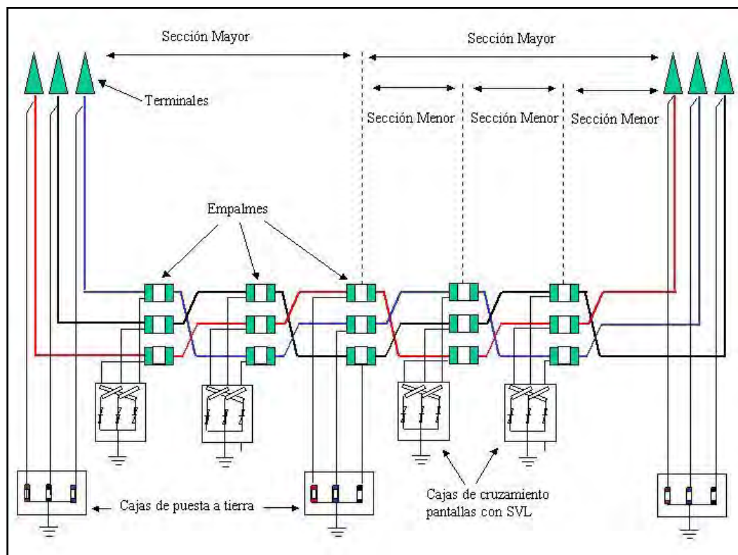
Figura 9: Pantallas cruzadas (cross bonding)
